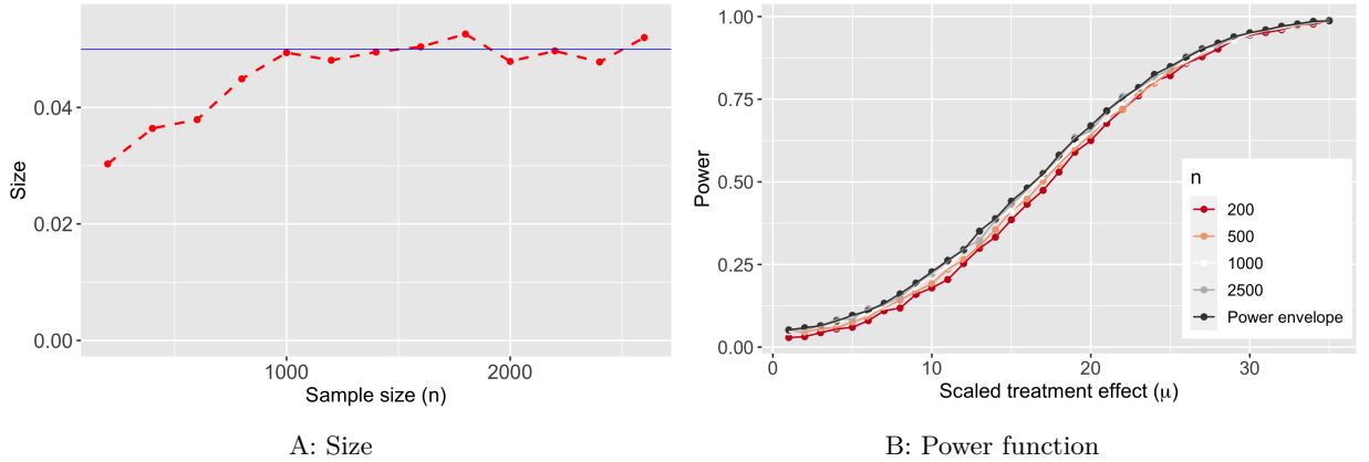
Note: Panel A plots the size of \hat{\varphi} at the nominal 5% level (solid blue line) when the errors are drawn from a \sqrt{3} \times \text{Uniform}[-1, 1] distribution for each treatment. Panel B plots the finite sample power envelopes for different n , along with asymptotic power envelope for unbiased tests. The scaled treatment effect is defined as \mu = \sqrt{n}|\delta| .
