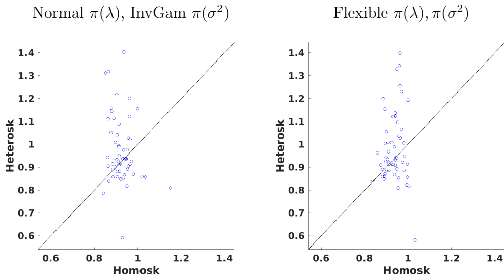
Figure 6: RMSE Ratios
