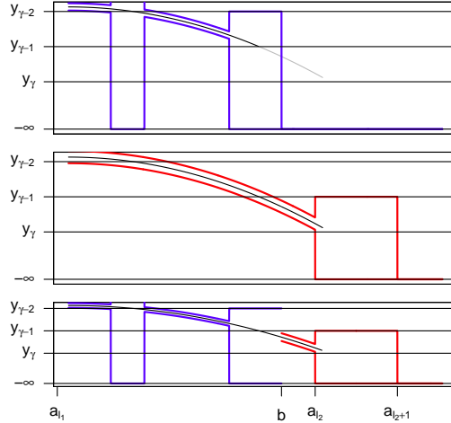
FIG 1. Theorem 4.1: Bracketing of a concave function \varphi (rather than h(\varphi) ). Here I_{i,\gamma}^L = [a_{i_1}, a_{i_2}] and I_{i,\gamma}^U = [a_{i_1-1}, a_{i_2+1}] , and the right boundary of the domain of \varphi lies between a_{i_2} and a_{i_2+1} . We focus on the right side, near a_{i_2} and a_{i_2+1} . In the top plot is a bracket on the domain \cup_{j=1}^{\gamma-1} I_{i,j}^U (which we let have right endpoint b here) and the range [y_{\gamma-1}, y_0] (below which \varphi is greyed out). The next plot shows an application of Proposition 4.1 to find a bracket on I_{i,\gamma}^L . The final plot shows the combination of the two.
