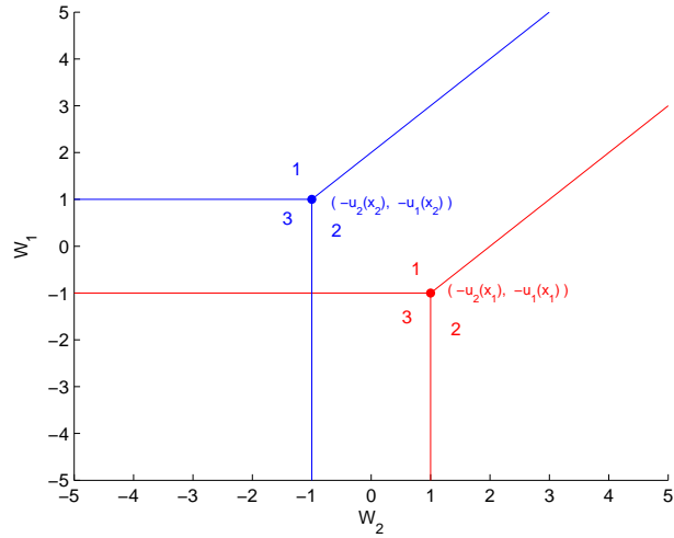
Figure 1: Orientations of w(x) = (-u_1(x), -u_2(x)) when M = 3 and K = 2 , cases 1a, 2a, and 3a.
