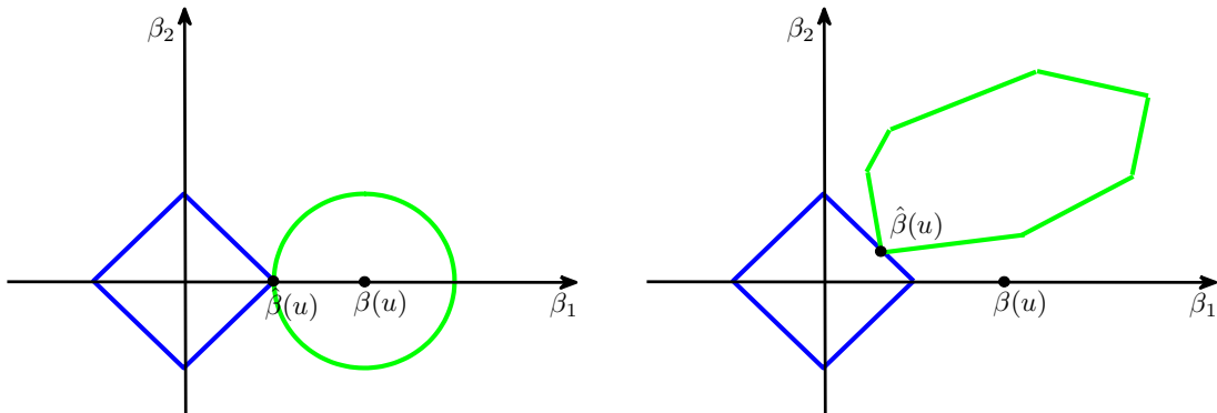
FIG 1. These figures provide a geometric illustration for the discussion given in the text concerning why \ell_1 -penalized estimation may be (left panel) or may not be (right panel) successful at selecting the minimal true model.
