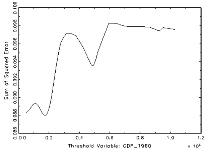
Figure 1: First Sample Split
