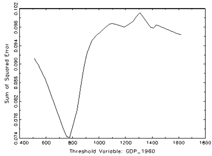
Figure 2: Second Sample Split
